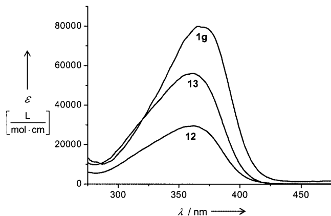
Figure 1. UV/Vis spectra of the mono-, di-, and tristyryl-substituted 1,3,5-triazines 12 , 13 , and 1g , respectively (measured in \text{CH}_2\text{Cl}_2 )
