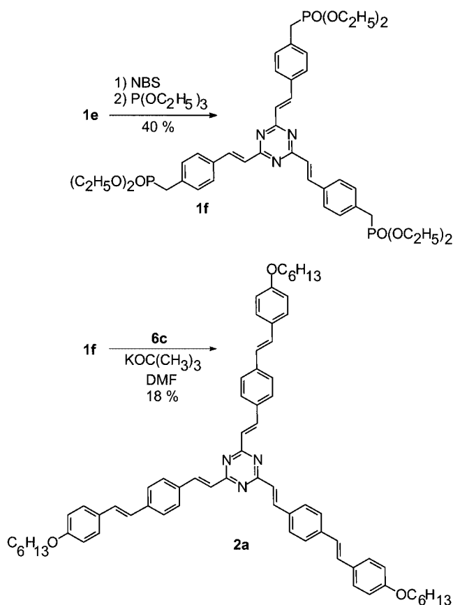
Scheme 3. Preparation of 2,4,6-tris[( E )-2-(4-{( E )-2-[4-(hexyloxy)phenyl]ethenyl}phenyl)ethenyl]-1,3,5-triazine ( 2a )
