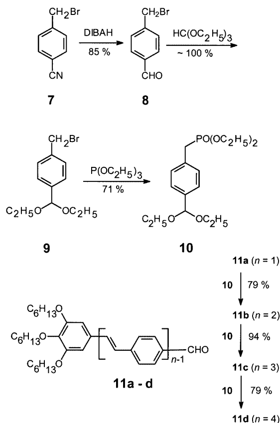
Scheme 4. Extension of the conjugated OPV chain in the series of the aldehydes 11a–d
