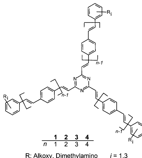
Scheme 1. Star-shaped compounds 1–4 having 1,3,5-triazine cores, which behave as electron acceptors, and OPV arms featuring terminal donor substituents
