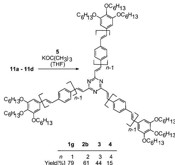
Scheme 5. Preparation of the 1,3,5-triazines 1g , 2b , 3 , and 4 having conjugated OPV arms and threefold terminal hexyloxy substitution
