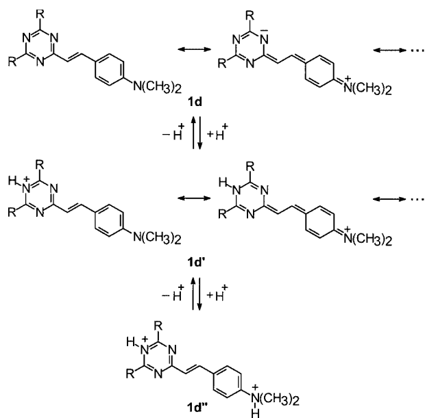
Scheme 7. Protonation of 1d in \text{CDCl}_3/\text{CF}_3\text{COOH} yields the violet species 1d' and the colorless form 1d'' (R represents the three equal arms of 1d , 1d' , and 1d'' )
