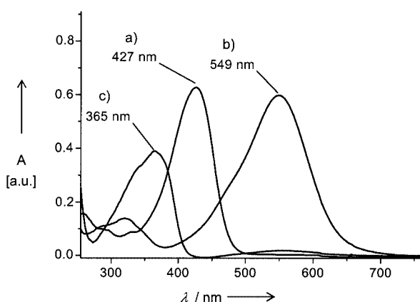
Figure 4. Protonation of 1d in \text{CHCl}_3/\text{CF}_3\text{COOH} : a) yellow, neutral, 5.068 \cdot 10^{-6} M solution of 1d in \text{CHCl}_3 ; b) violet solution of 1d' (4-fold excess of TFA); and c) colorless solution of 1d'' (20-fold excess of TFA)
