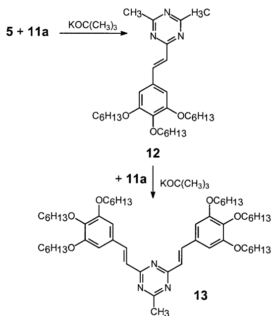
Scheme 6. Stepwise condensation of 5 and 11a to yield 12 and 13
