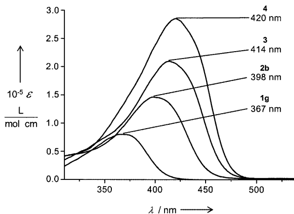
Figure 2. UV/Vis spectra of the series 1g , 2b , 3 , and 4 in \text{CH}_2\text{Cl}_2
